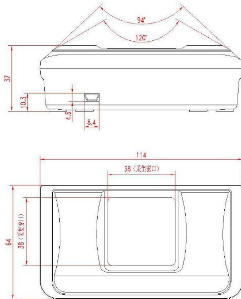
Fig 1. Size of the fingerprint scanner.
